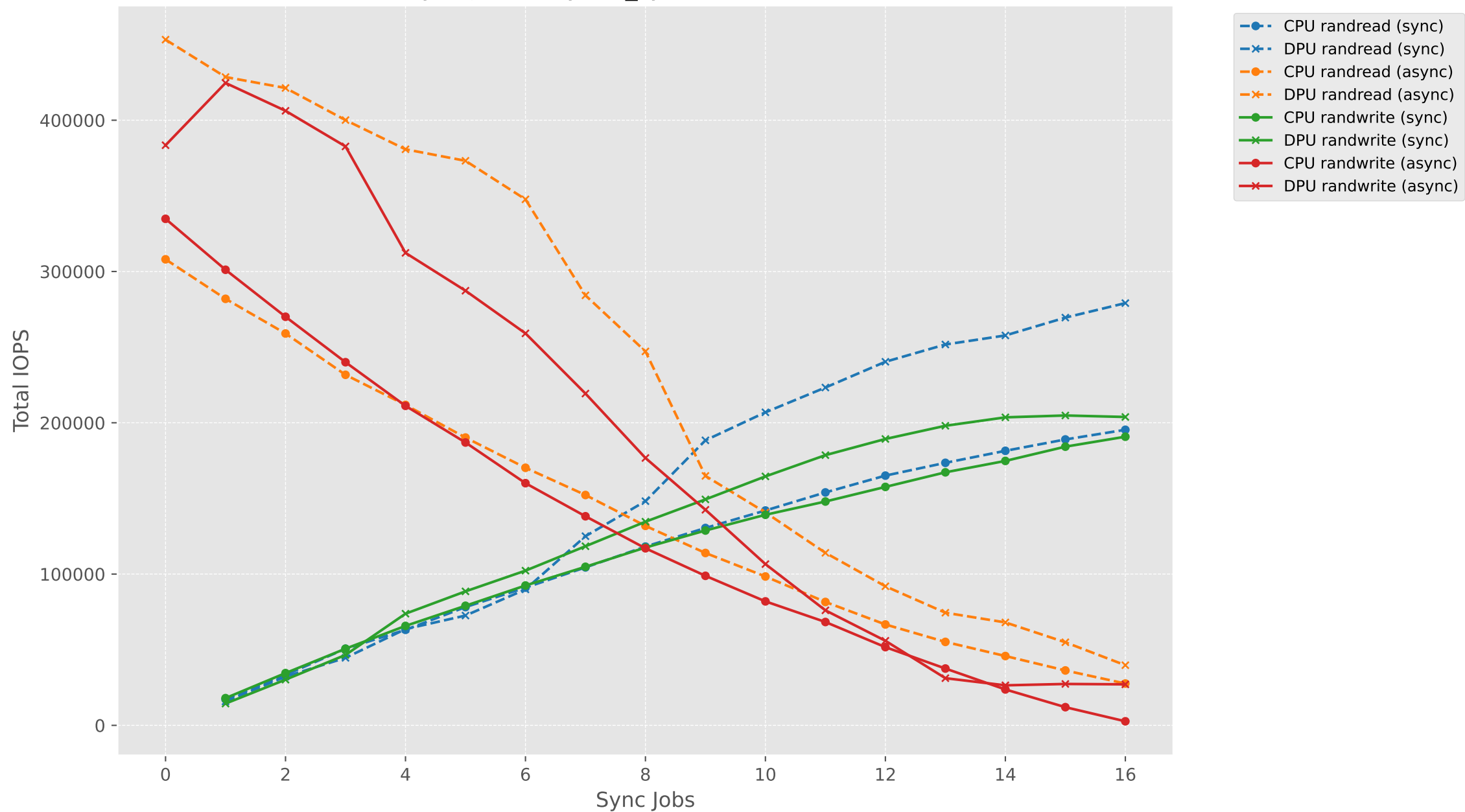
IOPS vs Sync Jobs (async1_syncN) - RAND (CPU vs DPU)
